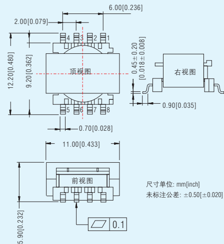
TTURA/B-6/10T 系列 LxWxH: 12.20x11.00x5.90(mm)
