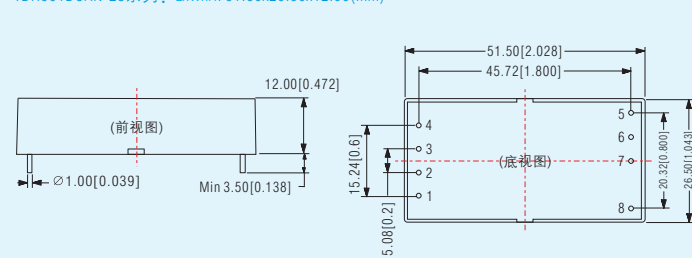
TDH501DCAN-ZC系列: LxWxH: 51.50x26.50x12.00(mm)
