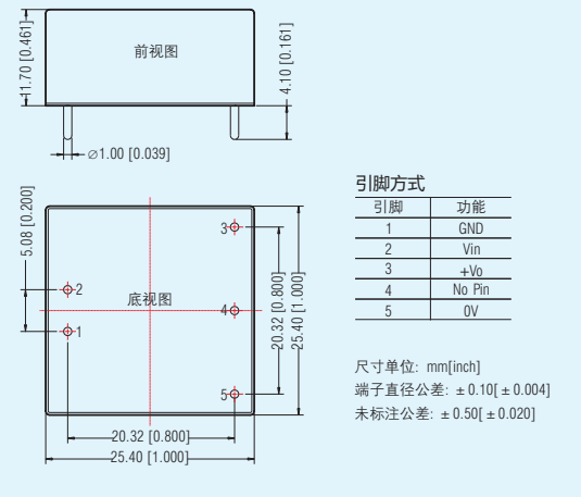
CUWB_YMD-6WR3系列 LxWxH: 25.40x25.40x11.70(mm)
