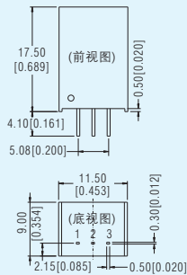
K78-1000R3, K78U-500, K78-1500 系列 LxWxH: 11.50x9.00x17.50(mm)
