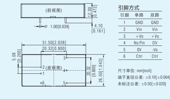
URE/F_LP-10WR3系列 LxWxH: 51.50x26.50x12.00(mm)
