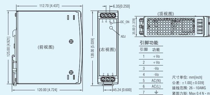
LI120-20BxxR2/LI120-13Bxx系列: LxWxH: 125.00x35.00x120.00(mm)
