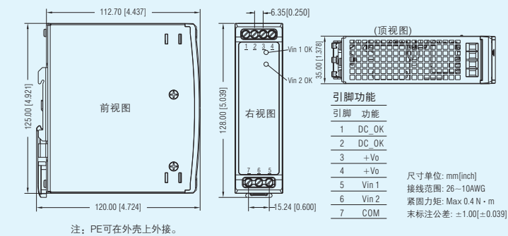
LIR-20: LxWxH: 125.00x35.00x120.00(mm)
