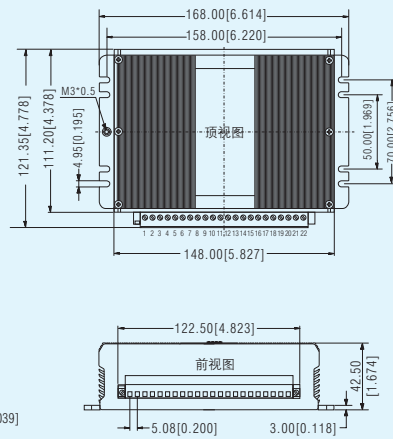
PV200-27B系列 LxWxH: 168.00x121.35x42.50(mm)
