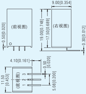
K78-1000R3L, K78U-500L, K78-1500L 系列 LxWxH: 19.00x11.50x9.00(mm)
