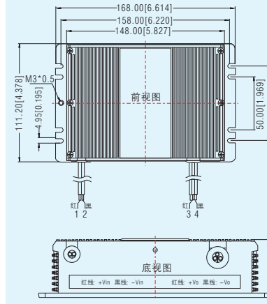
PV150-29Bxx系列 LxWxH: 168.00x111.20x42.50(mm)
