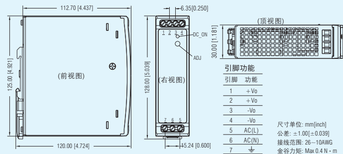
LI75-20BxxR2系列: LxWxH: 125.00x30.00x120.00(mm)
