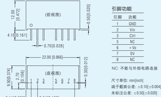
VRB-S-10WR3、URB-S-10WR3 系列 LxWxH: 22.00x9.50x12.00(mm)
